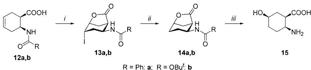
Scheme 3. (i) KI, I 2 , NaHCO 3 , CH 2 Cl 2 , 20 h, room temp.; (ii) Bu 3 SnH, CH 2 Cl 2 , 20 h, 40 °C; (iii) 20% HCl, 30 h room temp.
