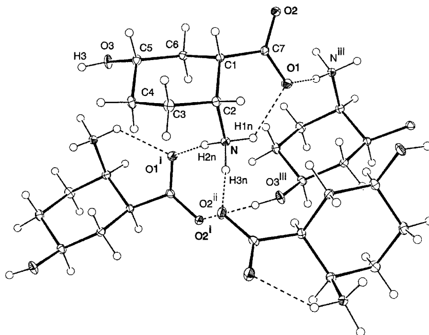
Figure 1. Crystal structure of 15 , showing the hydrogen bonding scheme. Thermal ellipsoids have been drawn at the 30% probability level. Symmetry codes: i = x + 1/2, -y + 3/2, -z + 2 , ii = -x + 3/2, -y + 1, z + 1/2 and iii = x + 1/2, -y + 3/2, -z + 1 .
