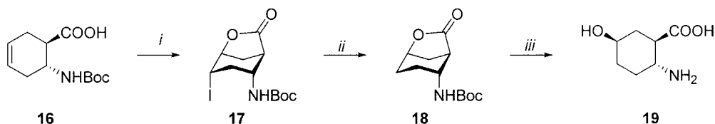
Scheme 4. (i) KI, I 2 , NaHCO 3 , CH 2 Cl 2 , 20 h, room temp.; (ii) Bu 3 SnH, CH 2 Cl 2 , 20 h, 40 °C; (iii) 20% HCl, 30 h, room temp.
