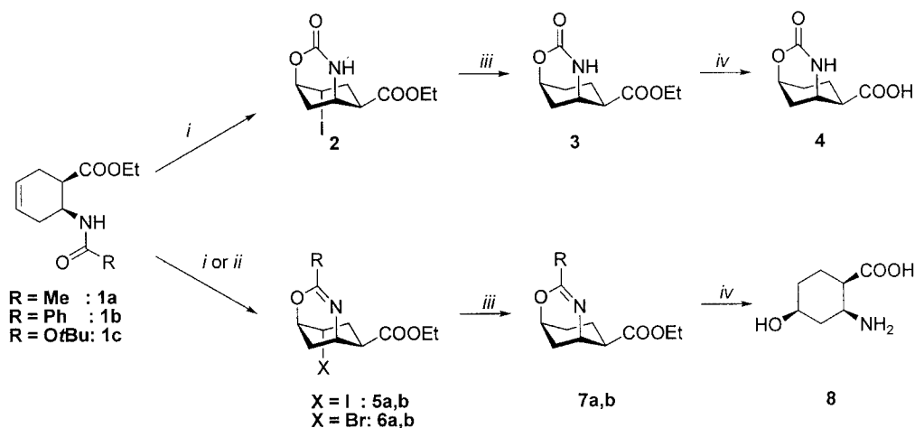
Scheme 1. (i) NIS, CH 2 Cl 2 , 14 h, room temp.; (ii) NBS, CH 2 Cl 2 , 14 h, room temp.; (iii) Bu 3 SnH, CH 2 Cl 2 , 20 h, 40 °C; (iv) 20% HCl, 30 h reflux.
