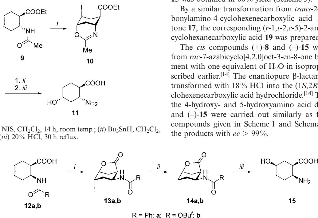
Scheme 3. (i) KI, I 2 , NaHCO 3 , CH 2 Cl 2 , 20 h, room temp.; (ii) Bu 3 SnH, CH 2 Cl 2 , 20 h, 40 °C; (iii) 20% HCl, 30 h room temp.
